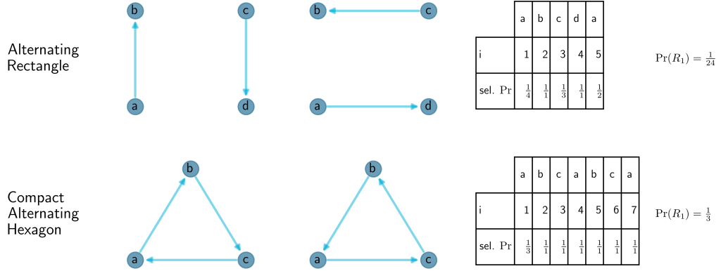
Figure 5: Examples of alternating cycles
