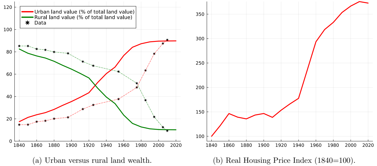
Figure 12: Land values and housing price.
