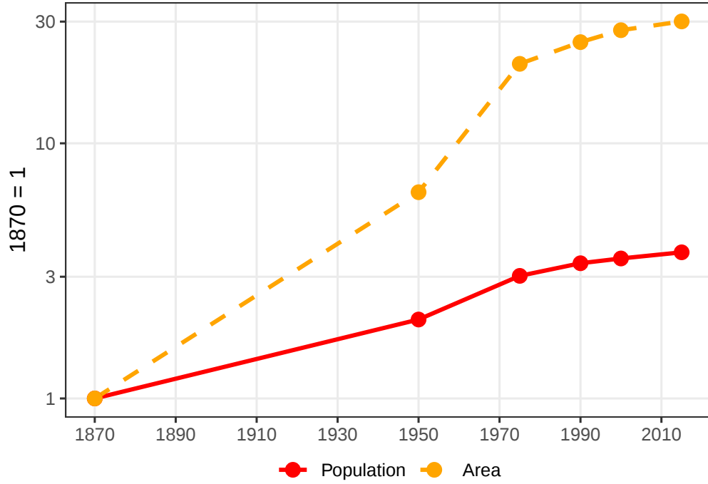
Figure 3: Urban area and population of the 100 largest cities in France (1870-2015).
