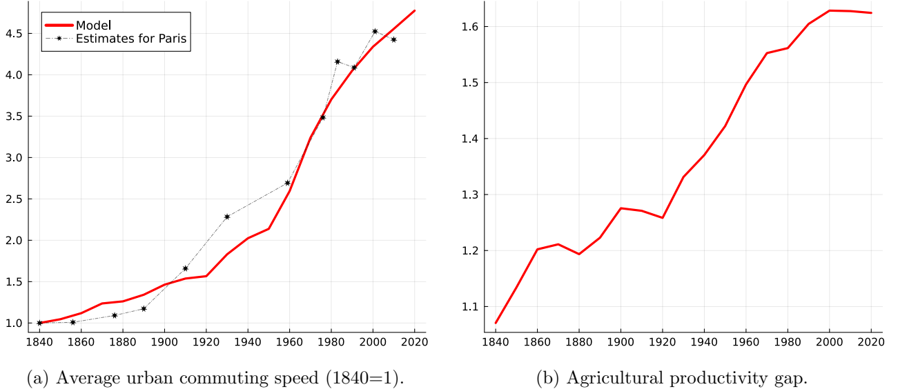
Figure 11: Commuting speed and the ‘agricultural productivity gap’.
