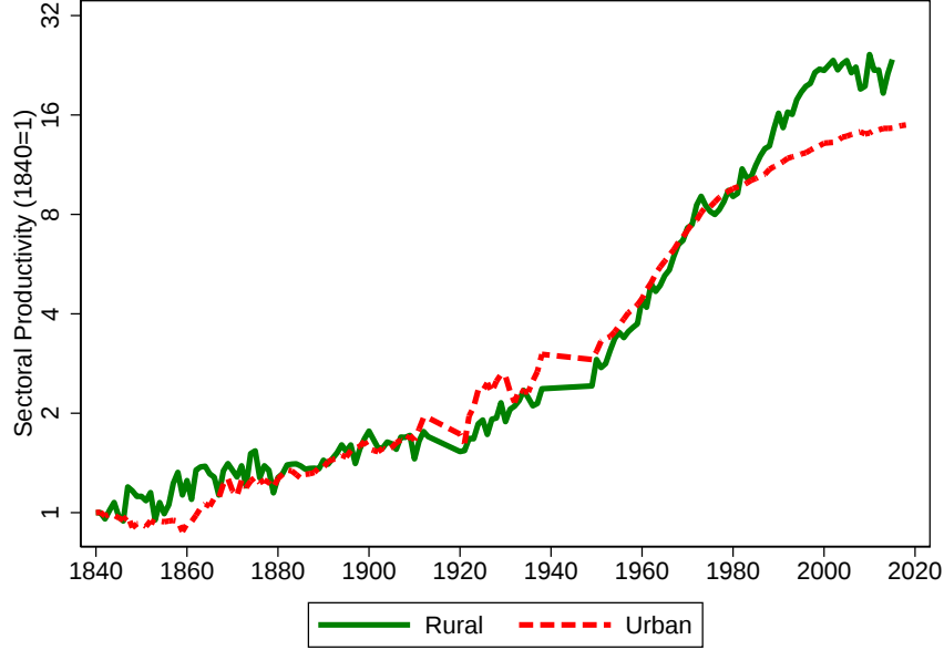
Figure 7: Estimated Aggregate Productivity Series, Rural ( \theta_{r,t} ) and Urban ( \theta_{u,t} ), 1840=1 (1840-2019). Estimation details in Appendix A.1.4.
