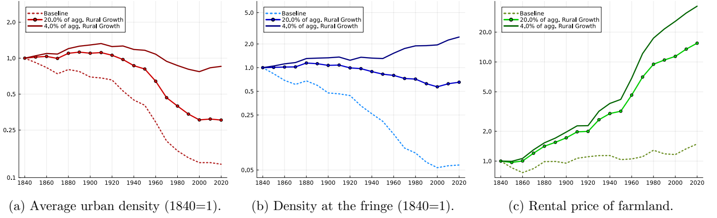
Figure 16: Sensitivity to rural productivity growth.
