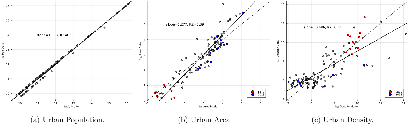
Figure 13: Regional Urban Moments.
