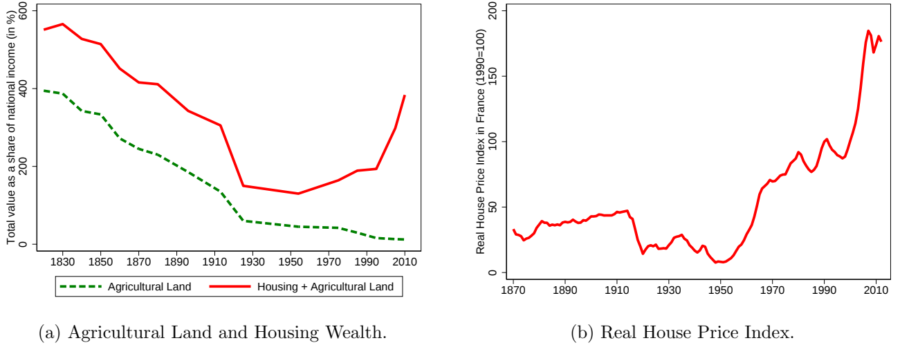
Figure 6: Land and Housing Values in France.
