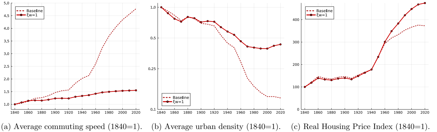
Figure 17: Sensitivity to the elasticity of commuting costs to income.
