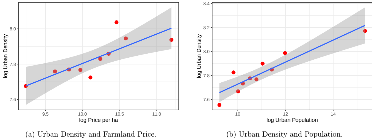
Figure 5: Urban density across French cities in 2000.
