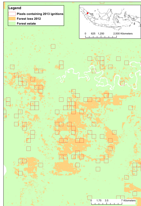
Figure 3: 2012 deforestation and 2013 ignitions in Riau
