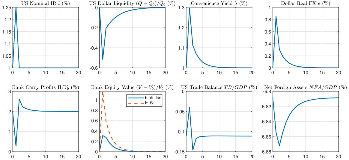
Figure 3: Impulse response to a U.S. monetary policy shock of 0.25%
