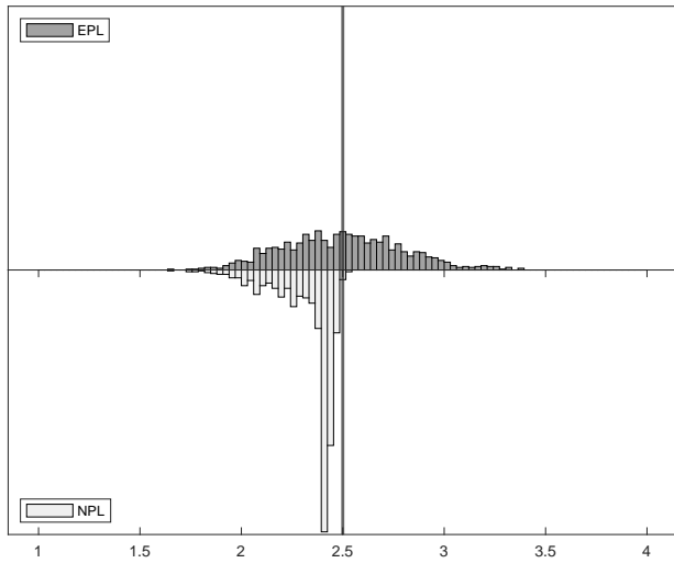
(b) Experiment 2: \hat{\theta}_{RN} when \theta_{RN} = 2.5
