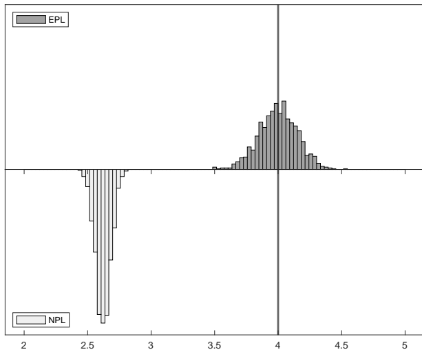
(c) Experiment 3: \hat{\theta}_{RN} when \theta_{RN} = 4
