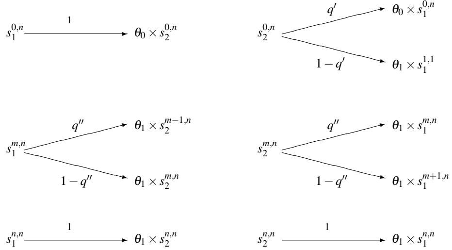
FIGURE 3 Type space for Example 8
