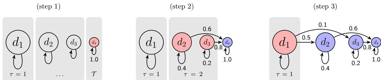
Figure 4: Graphical illustration of state recursion on the DAG D(\mathcal{G}) in Example 2.
